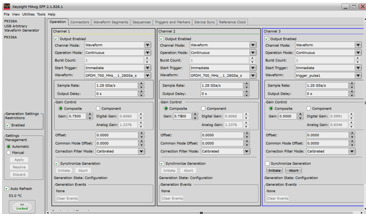
Figure 4. P9336A AWG soft front panel
